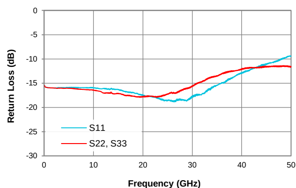
Return Loss
